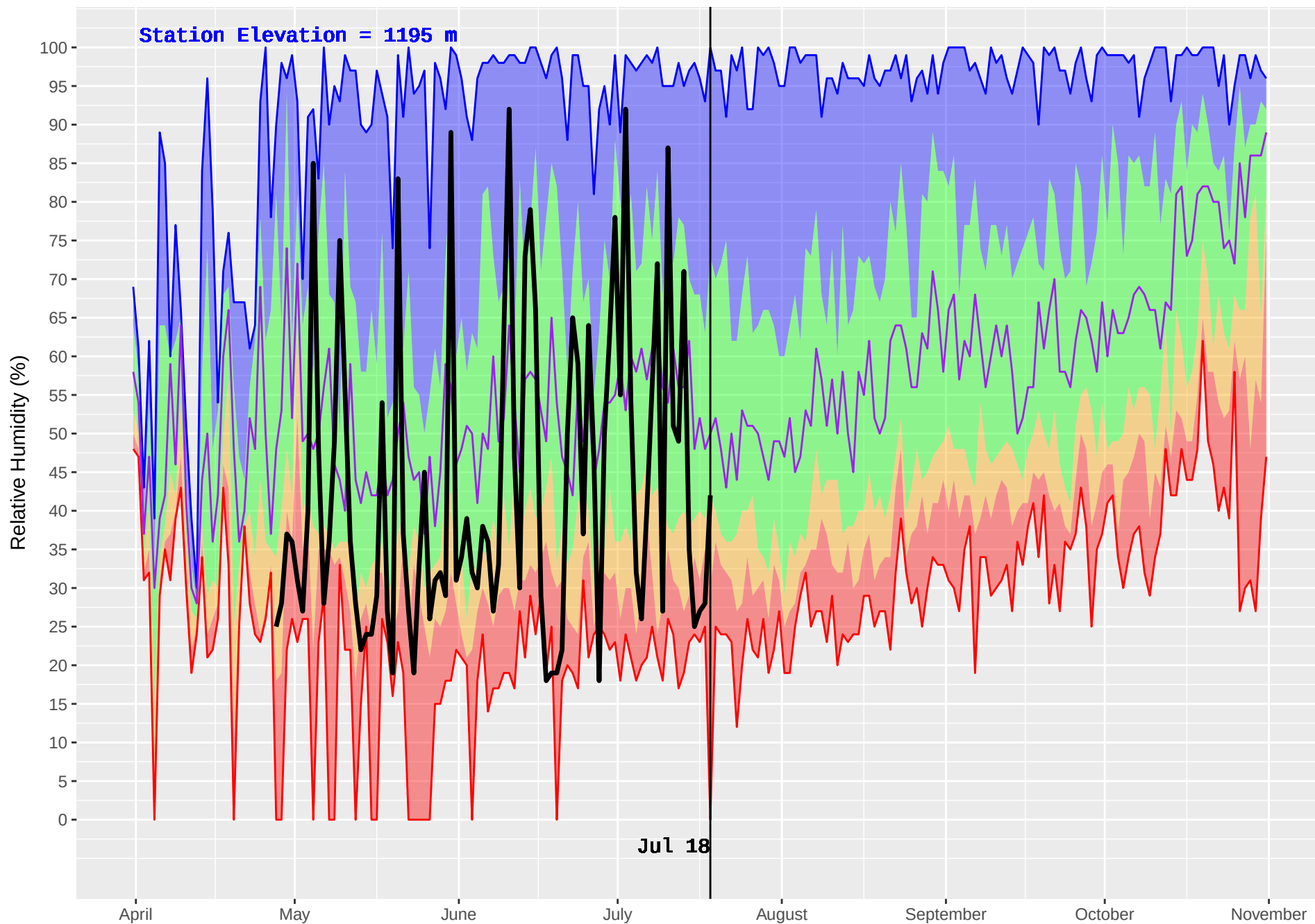
VALEMOUNT 2 (200) : Historical (1986–2016) and Current (2018) Daily Relative Humidity
