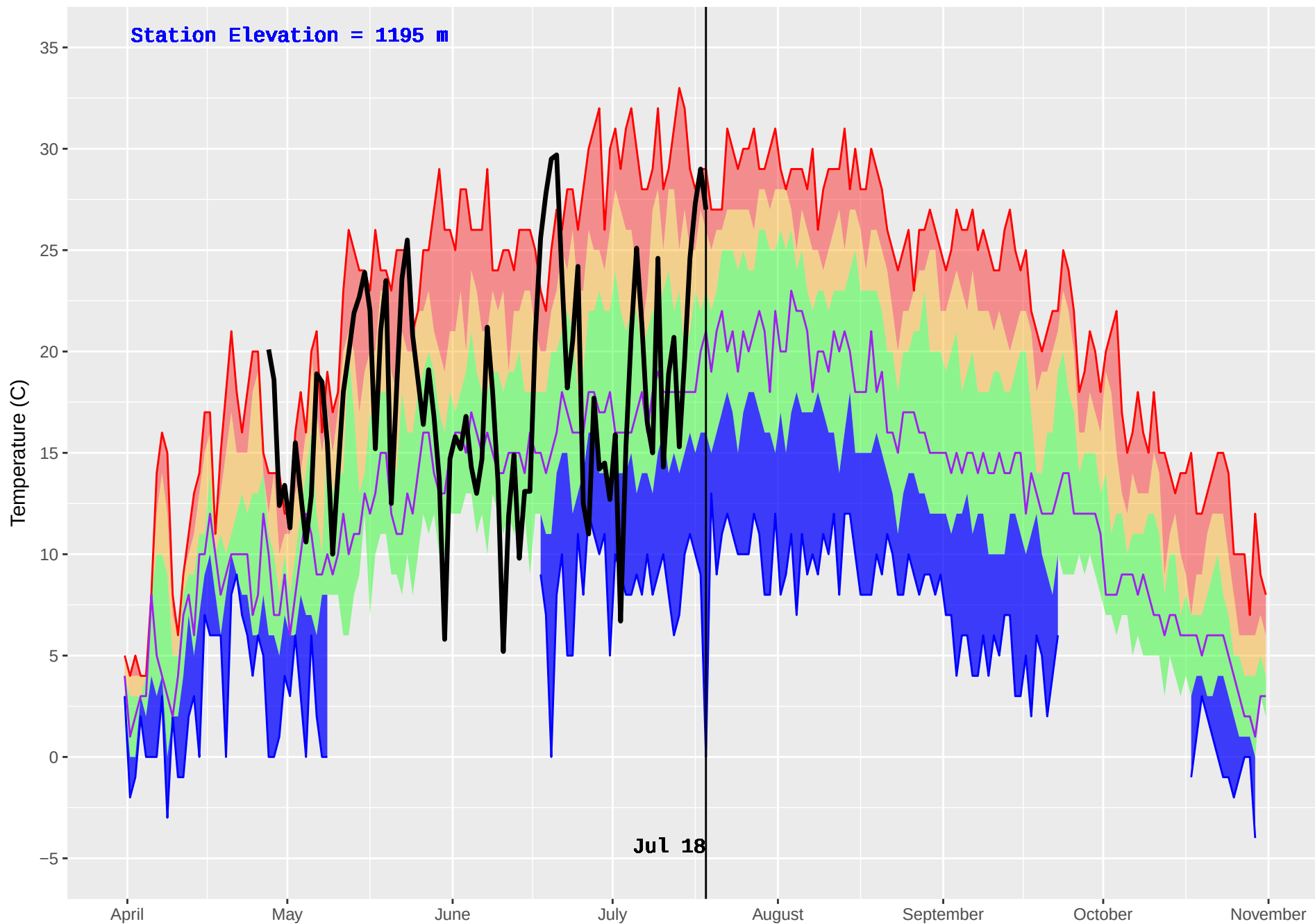
VALEMOUNT 2 (200) : Historical (1986–2016) and Current (2018) Daily Temperature
