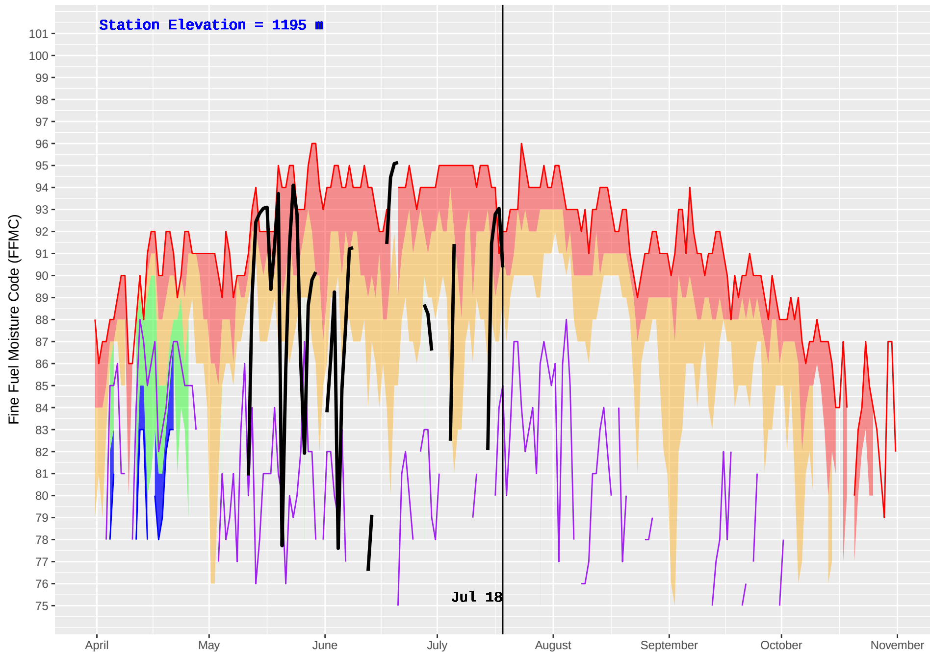
VALEMOUNT 2 (200) : Historical (1986–2016) and Current (2018) Daily Fine Fuel Moisture Code (FFMC)
