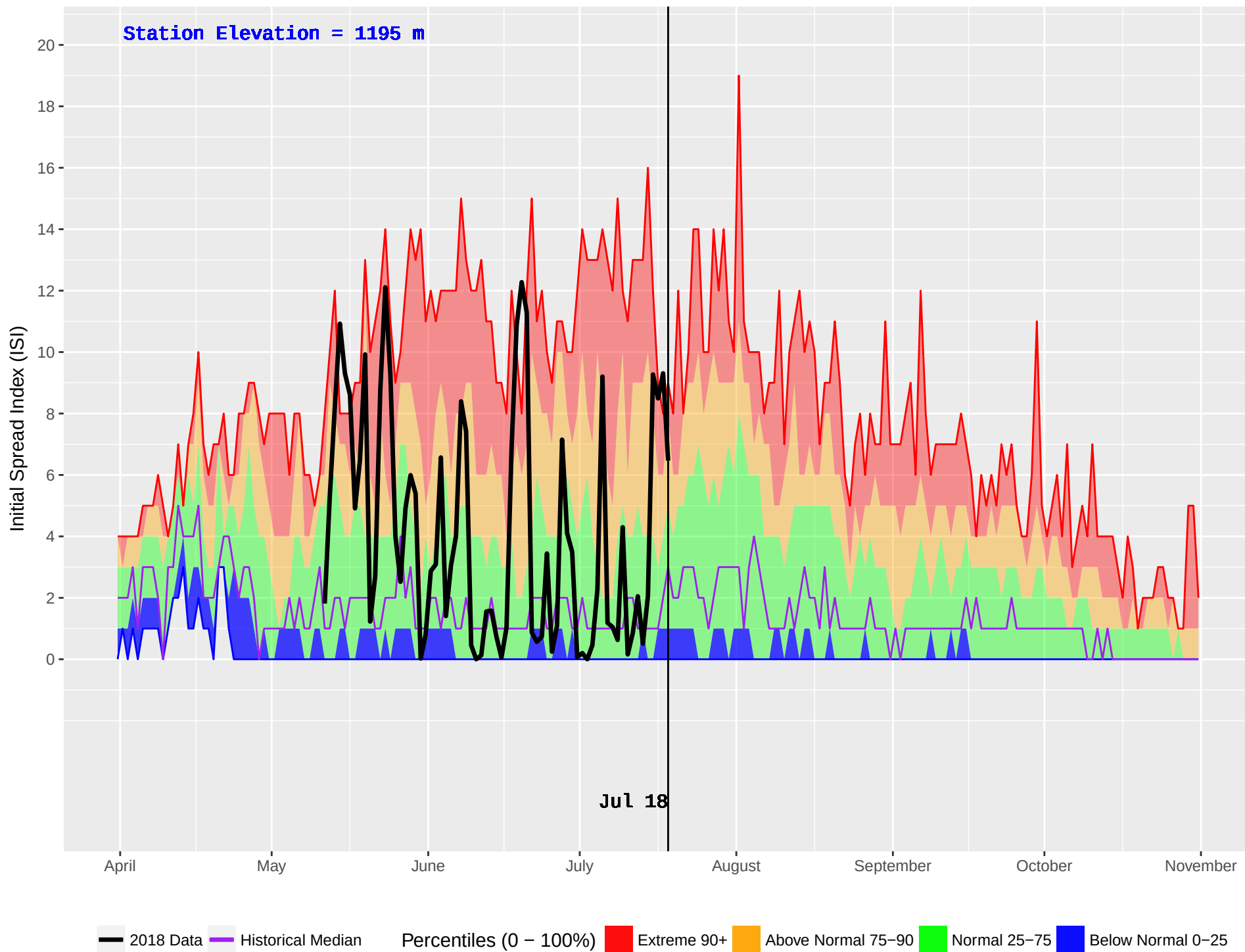
VALEMOUNT 2 (200) : Historical (1986–2016) and Current (2018) Daily Initial Spread Index (ISI)
