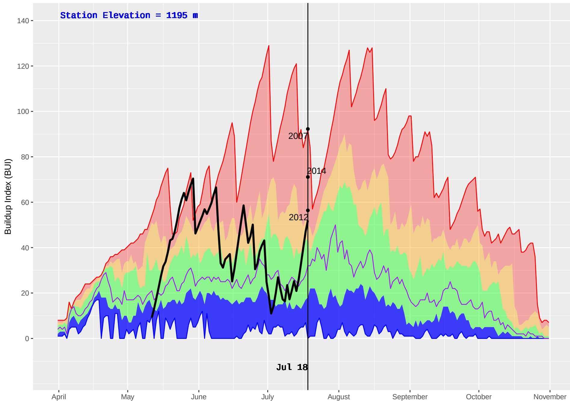
VALEMOUNT 2 (200) : Historical (1986–2016) and Current (2018) Daily Buildup Index (BUI)
